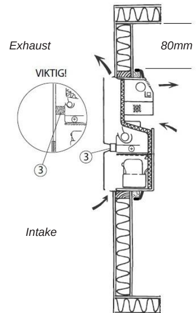
Cross-section. See detail 3
